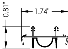
8A ARTICULATING SWEEP
